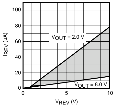
REVERSE BIAS CURRENT RANGE (V<sub>IN</sub> = 0 V)
