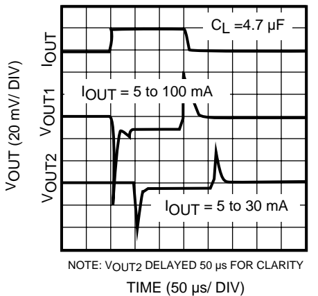
LOAD CURRENT STEP RESPONSE 1
